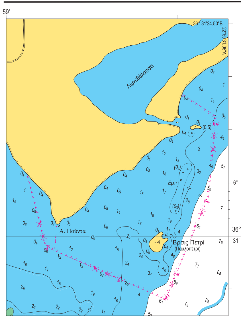
Block (A) for Inset ΣΤ1 "ELAFÓNISOS HARBOUR" Chart No 222/1
